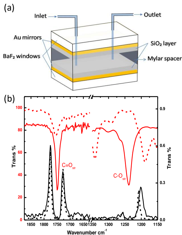
Figure 2. (a) Schematic representation of a flow cell FP cavity. (b) IR transmission spectra of 10 % EtOAc (red trace) and ATR spectrum of neat PNPA (dotted red trace). Vibro-polaritonic states P + and P - formed by coupling to the 10 th and 7 th cavity modes to carbonyl and acyl bands of EtOAc respectively (black trace; path-length is approx. 18 \mu m); dotted black trace represent the corresponding TMM simulation.
