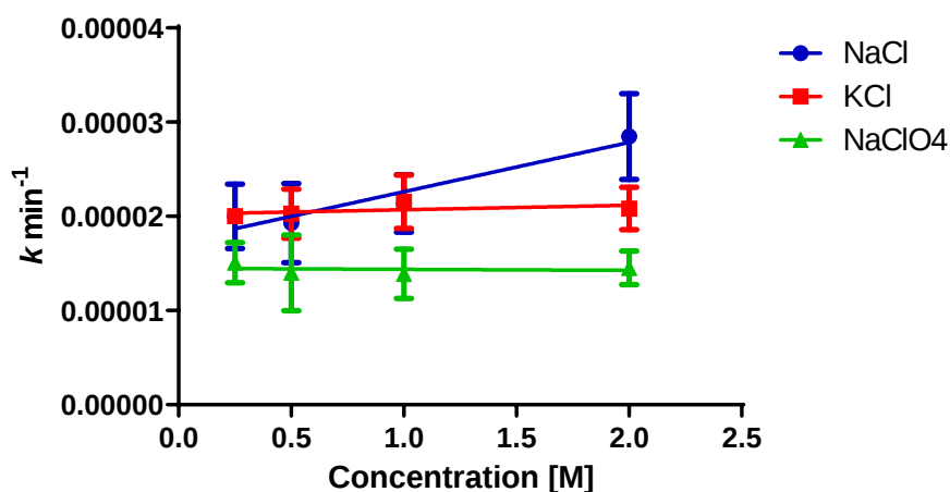
Figure S3. Salt effect upon rates of hydrolysis of PNPGlc in the pH-independent region pH 6.8 at 90 °C. Calculation of salt effect by plotting rate k \text{ min}^{-1} as a function of salt concentration of three different salts, KCl, NaCl, and NaClO 4 , k_{\text{KCl}} = 4.74 \times 10^7 \text{ min}^{-1} \text{ M}^{-1} , k_{\text{NaCl}} = 5.23 \times 10^6 \text{ min}^{-1} \text{ M}^{-1} , k_{\text{NaClO}_4} = -1.08 \times 10^7 \text{ min}^{-1} \text{ M}^{-1} .
