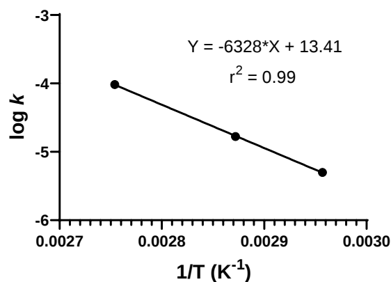
Figure S5. Arrhenius plot for the hydrolysis reaction of PNP-Glc in the pH independent region (pH 5.8).
