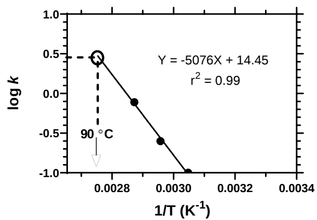
Figure S8. Arrhenius plot for the hydrolysis reaction of PNP-Glc in the strongly basic region (pH 12.42).
