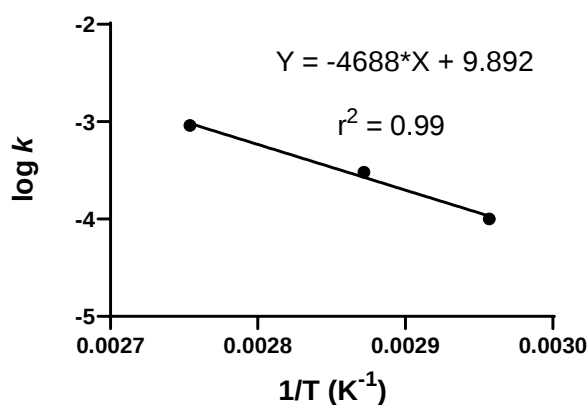
Figure S6. Arrhenius plot for the hydrolysis reaction of PNP-Glc in the weakly basic region (pH 8.55).
