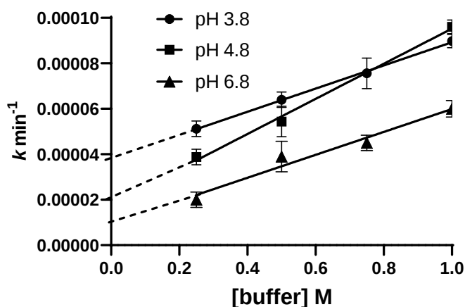
Figure S4. Buffer effect in the pH-independent region at 90 °C. Extrapolation to zero buffer across the pH-independent region as a function of buffer concentration at three different pH, 3.8, 4.8 and 6.8.
